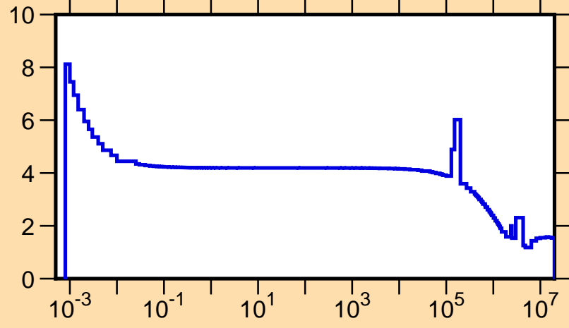
\sigma vs. E for ^{13}\text{C}(n,\text{tot.})
