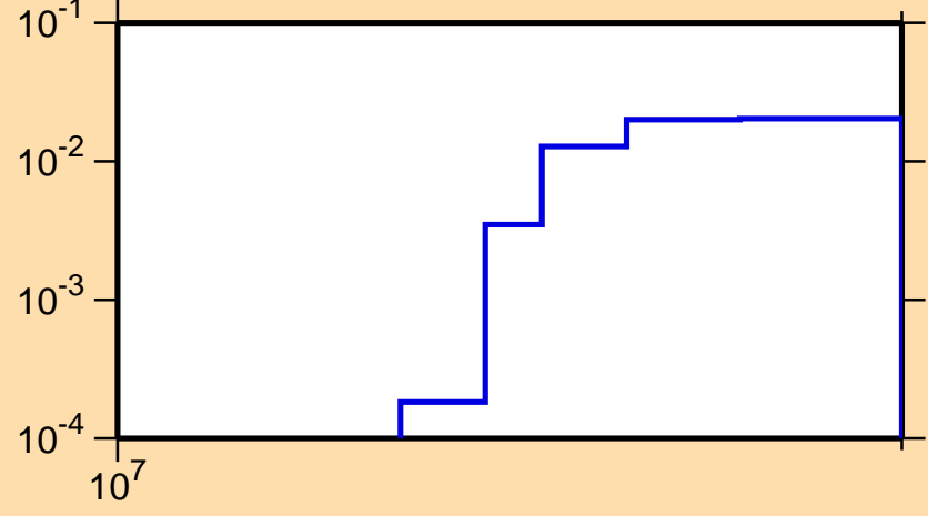
\sigma vs. E for ^{13}\text{C}(n,t)
