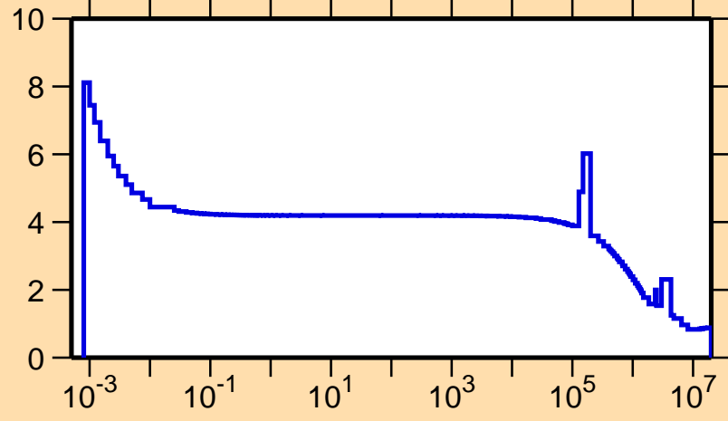
\sigma vs. E for ^{13}\text{C}(n,\text{el.})
