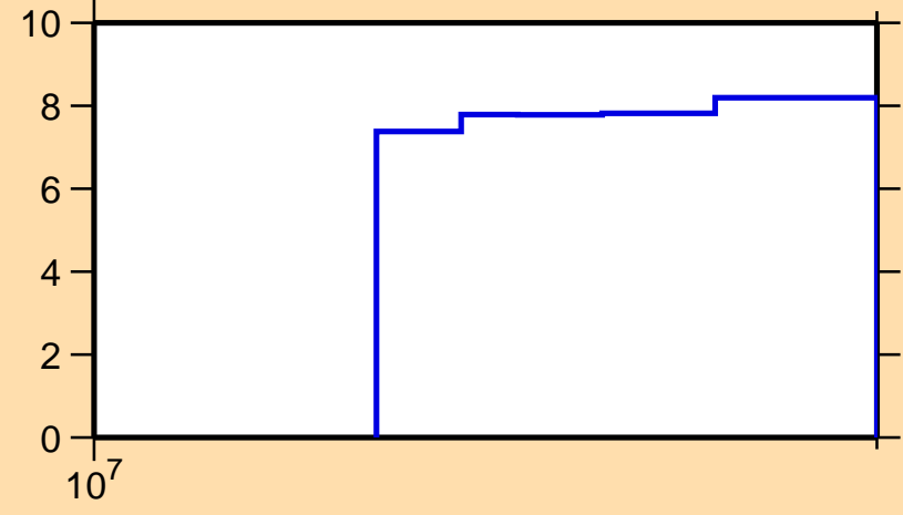
\Delta\sigma/\sigma vs. E for ^{13}\text{C}(n,el.)
